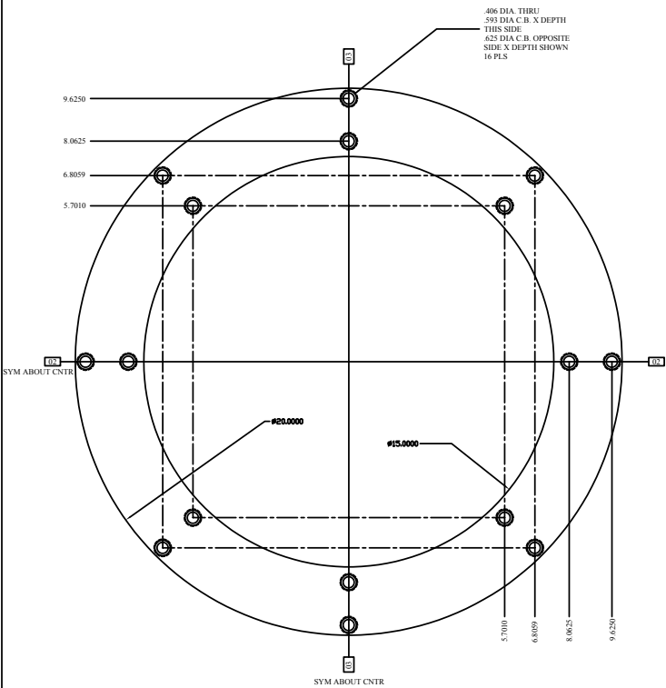
DETAIL 2 1 REQD. MTL. 6061 ALUMINUM
