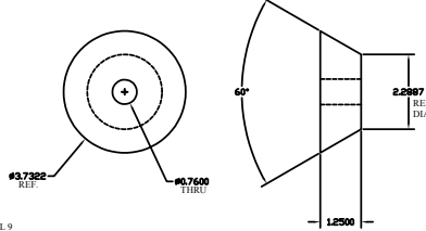
DETAIL 9 1 REQD. MTL. MILD STEEL
