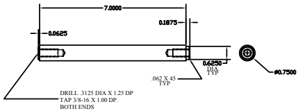
DETAIL 14 24 REQD. MTL. 6061 ALUMINUM
