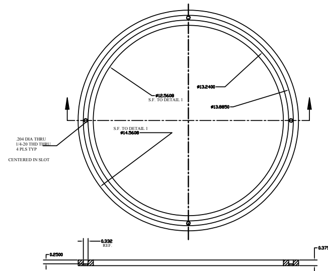
DETAIL 13A 1 REQD. MTL. 6061 ALUMINUM
